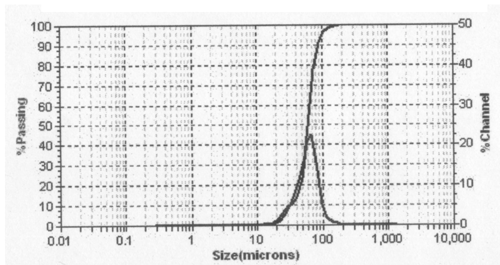
Microtrac 3500S
