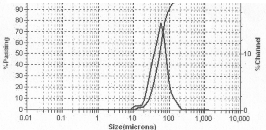
Microtrac 3500S
